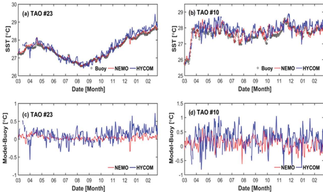
Fig. 3. Time series for daily mean SST of NEMO, HYCOM, and buoy at the two TAO buoys, (a, c) 23 and (b, d) 10, from March 2015 to February 2016 and the differences (c, d) between model and buoy.
