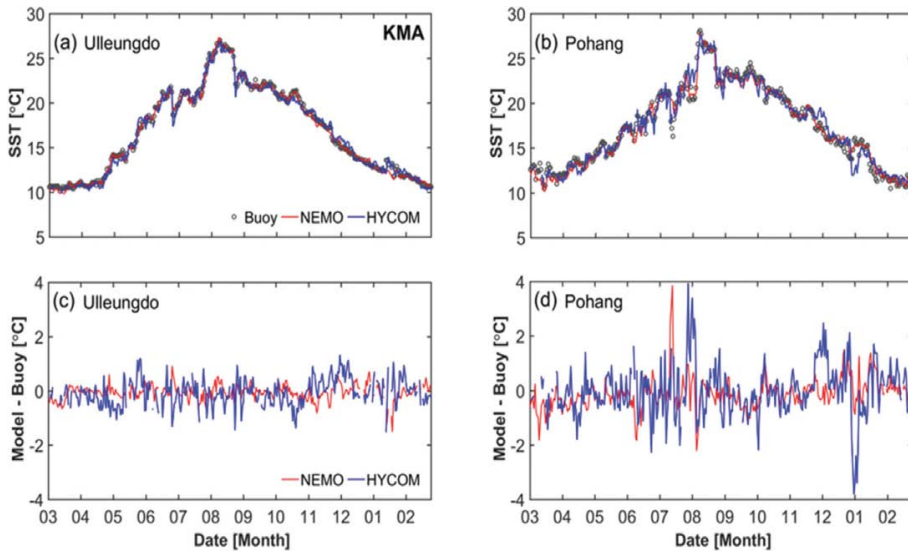
Fig. 9. Time series for daily mean SST of NEMO, HYCOM, and buoy at the two KMA buoys, (a, c) Ulleungdo and (b, d) Pohang buoy, from March 2015 to February 2016, and the differences (c, d) between model and buoy.
