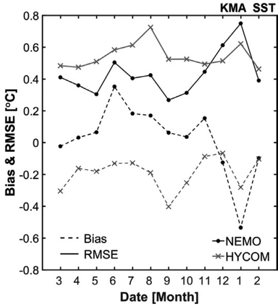
Fig. 10. Same as in Fig. 4, but using the eight KMA buoys.
