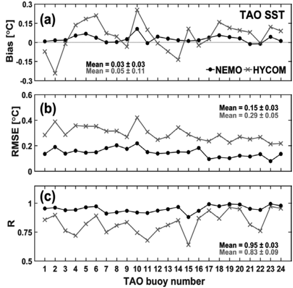
Fig. 2. Comparisons between NEMO and HYCOM for mean (a) Bias, (b) RMSE and (c) R at each TAO buoy. The black and gray lines represent NEMO and HYCOM, respectively.
