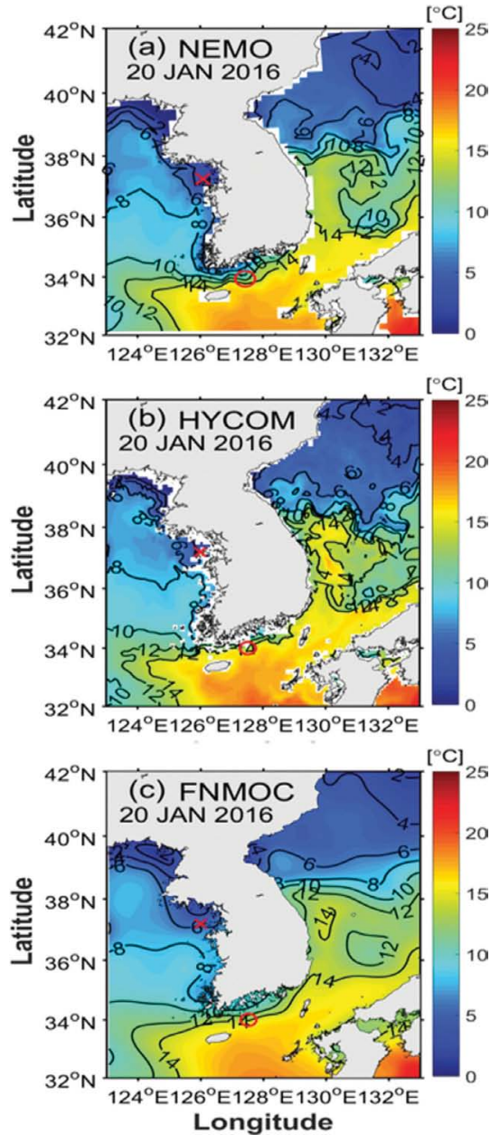
Fig. 12. Spatial distributions of SST from (a) NEMO, (b) HYCOM and (c) FNMOC satellite on 20 January 2016. The red X and O symbols represent the location of Deokjeokdo and Geomundo buoy. The contour interval is 2.0°C.
