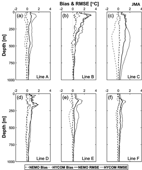
Fig. 7. Same as in Fig. 5, but at the six JMA ship observation lines.
