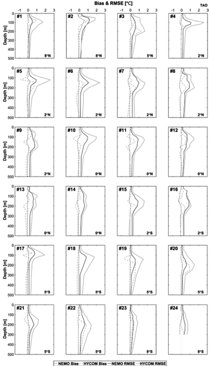
Fig. 5. Comparisons between NEMO (black) and HYCOM (gray) for mean Bias (dashed line) and RMSE (bold line) at each TAO buoy, which are estimated according to depth using vertical temperature profile.
