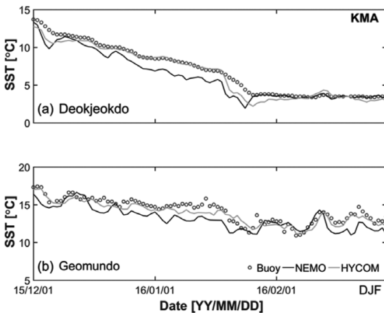
Fig. 11. Same as in Fig. 9, but at the two KMA buoys, (a) Deokjeokdo and (b) Geomundo buoy, during the winter season (December 2015 to February 2016).
