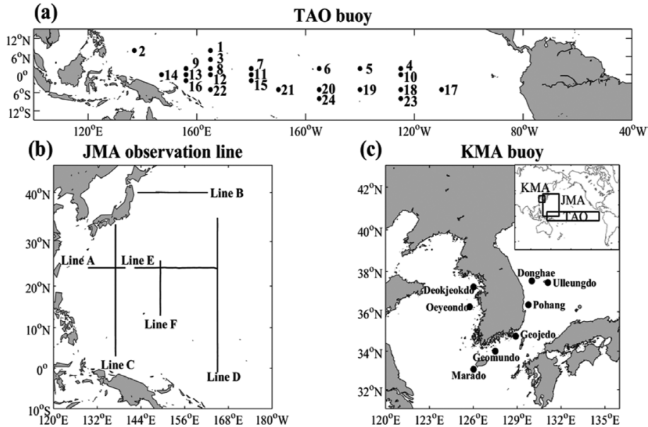
Fig. 1. Locations of (a) TAO buoy, (b) JMA ship observation line and (c) KMA buoy.
