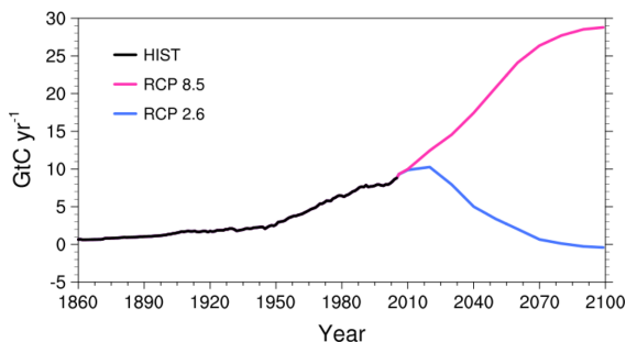
Fig. 1. Carbon dioxide emissions (GtC yr -1 ) used in the experiment of this study from 1860 to 2100. RCP 2.6 and 8.5 are marked in blue and red.
