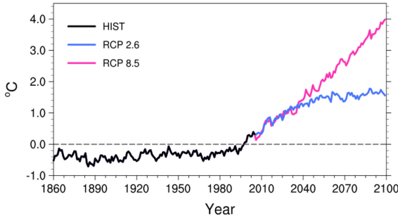
Fig. 3. Global mean temperature changes ( ^{\circ}\text{C} ) relative to 1985~2005 baseline period in emission-driven run from 1860 to 2100. Historical period is in black and RCP colors are as indicated.
